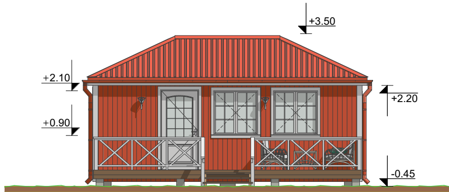
FASAD A
